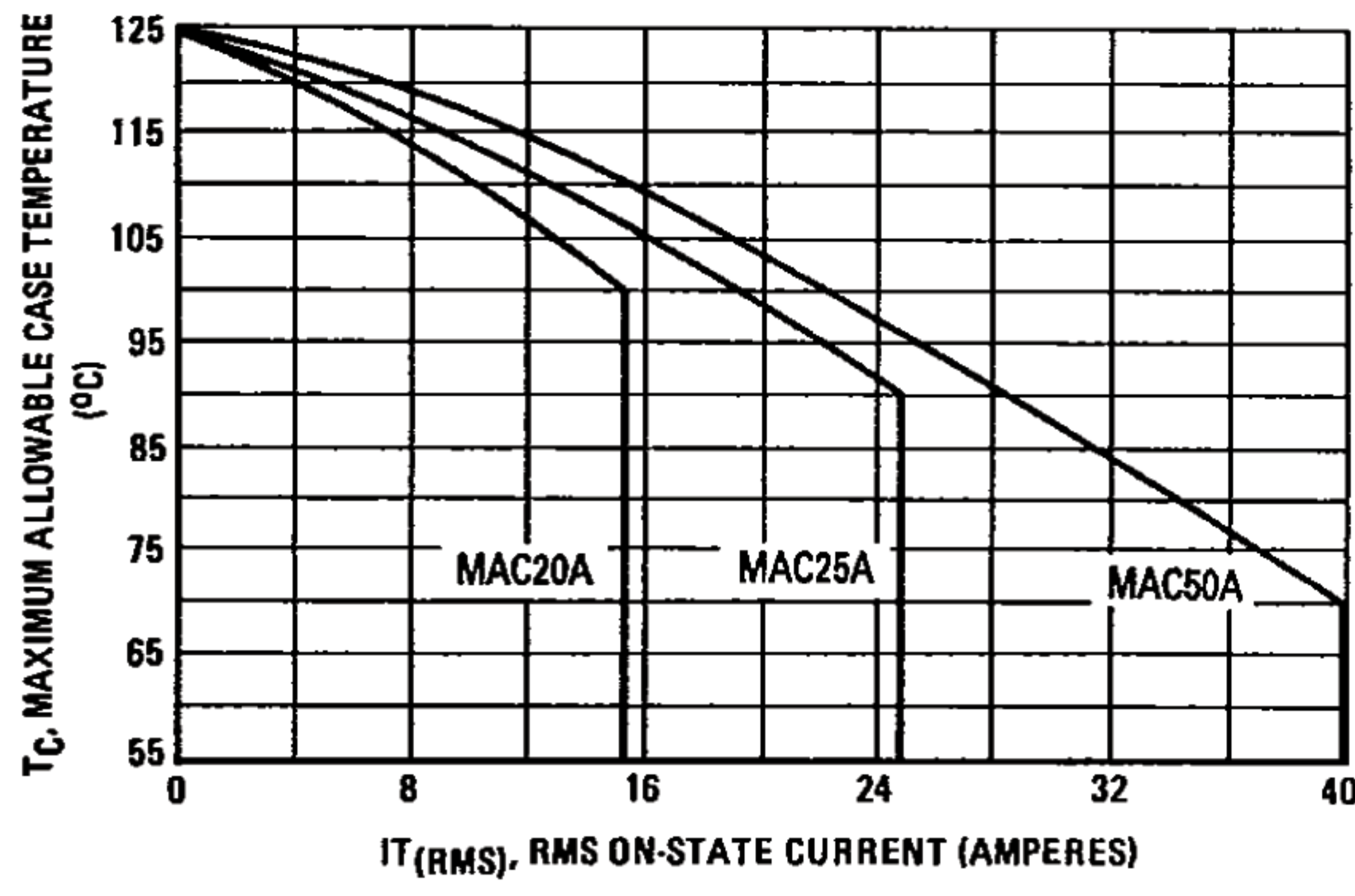
FIGURE 1 – CURRENT DERATING
